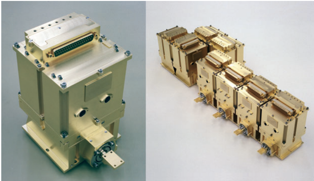
Fig. 3-8: Single SCIAMACHY detector module (left) and the full complement of 8 detector modules (right). (photo: SRON)
