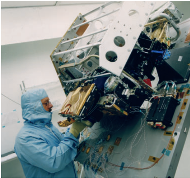
Fig.3-13: Integration of the OA. (photo: Dutch Space)
