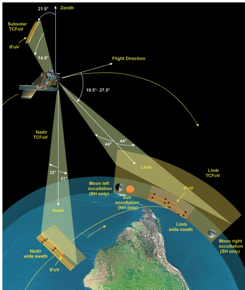
Fig. 3-5: Sketch of SCIAMACHY's TCFoV and observation geometries. (graphics: DLR- IMF)
