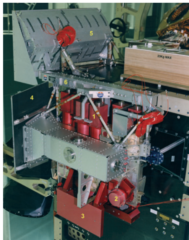
Fig. 3-12: Structural Model of the OA showing the SCIAMACHY design with detectors (1), ESM with Nadir Calibration Window (2), nadir baffle (3), RAD A (4), SRC (5) and Thermal Bus (6). (photo: ESA)
