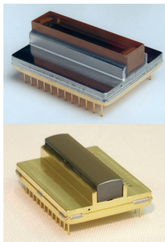
Fig. 3-7: The RETICON (top) and EPITAXX (bottom) linear detector arrays. (photo: SRON)
