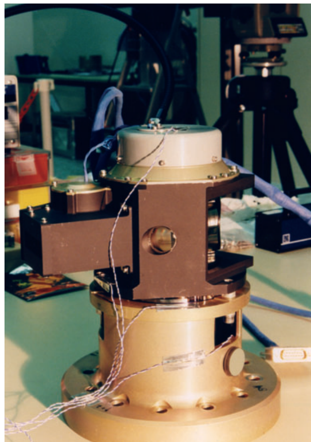
Fig. 3-6: ESM scanner on vibration test adaptor. The left-most rectangular opening is the Nadir Calibration Window. (photo: EADS Astrium)
