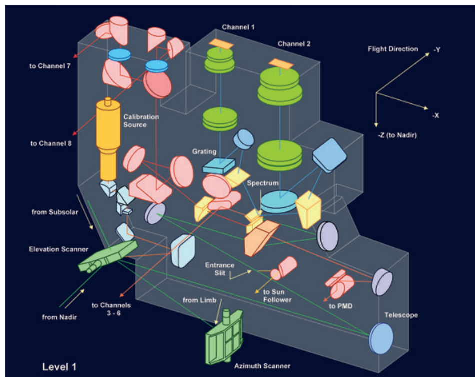
Fig. 3-2: Optical configuration level 1. (graphics: DLR-IMF, modified after SJT 1996)
