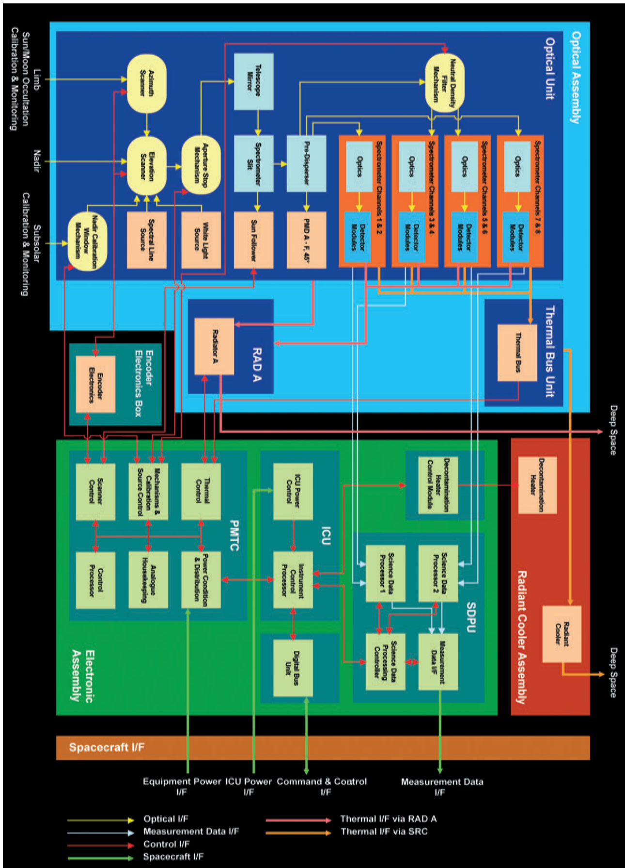
Fig.3-1: SCIAMACHY functional block diagram with simplified interfaces between assemblies and modules. (graphics: DLR-IMF, modified after EADS Astrium 2004)
