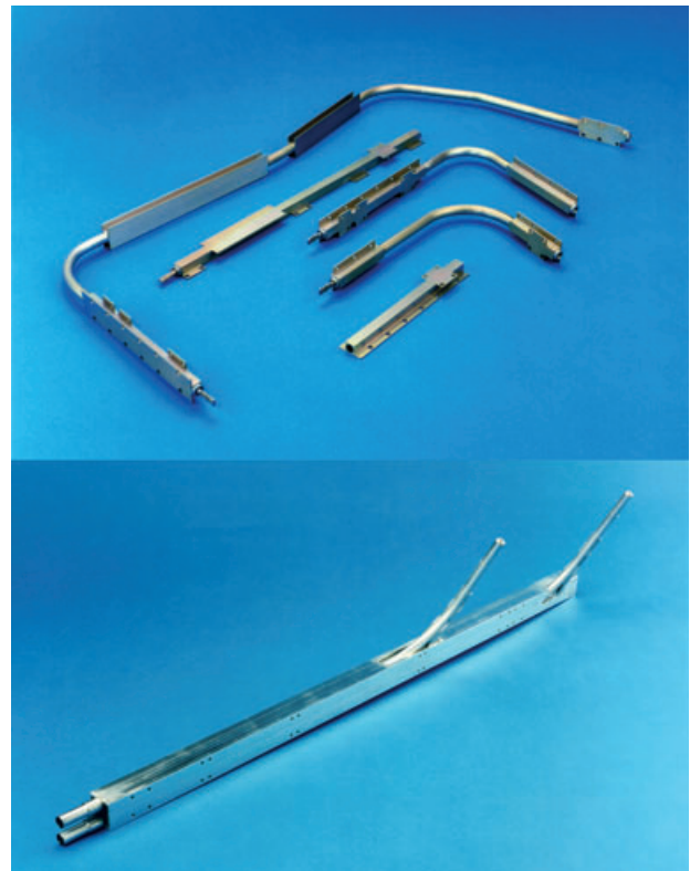
Fig. 3-10: Heat pipes from optical bench to RAD A (top) and cryogenic heat pipes from detectors 7 & 8 to SRC (bottom). (photo: EADS Astrium)
