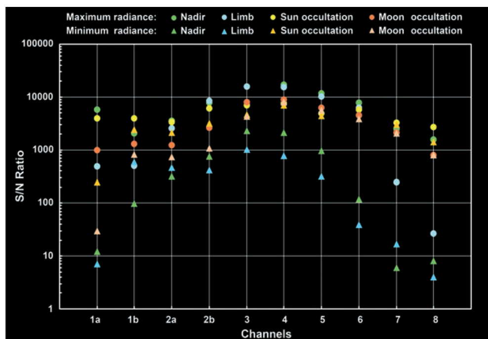
Fig. 3-9: The signal-to-noise ratios for all channels as obtained during OPTEC-5 tests. The ratios were determined for minimum and maximum radiance signals. (graphics: DLR-IMF)
