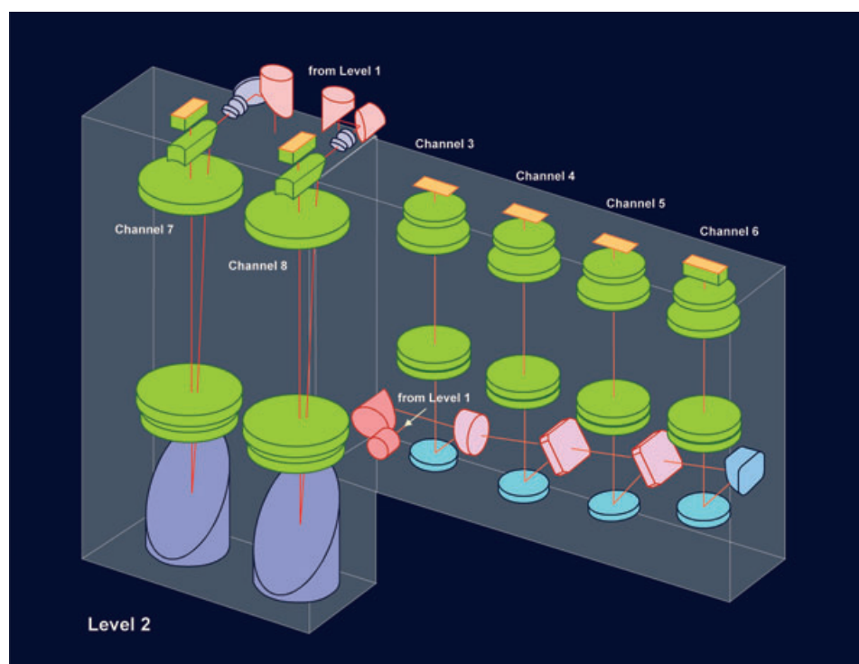
Fig. 3-3: Optical configuration level 2. (graphics: DLR-IMF, modified after SJT 1996)
