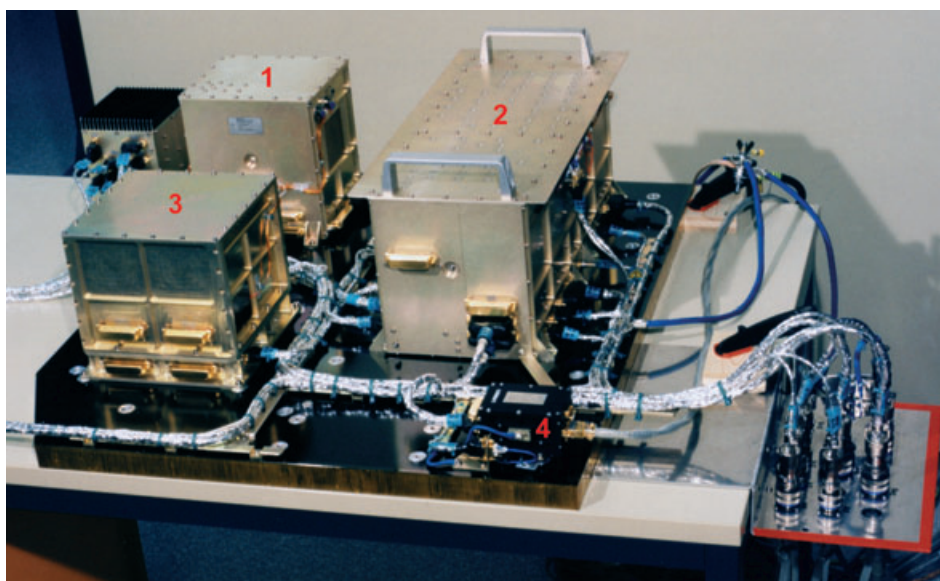
Fig.3-11: The Simplified Engineering Model of the EA with ICU (1), PMTC (2), SDPU (3) and DBU (4). (photo: EADS Astrium)
