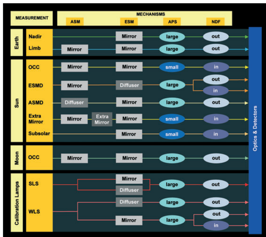
Fig. 3-4: SCIAMACHY optical 'trains'. Each 'train' defines a path for the measured light through the instrument to the detectors. Light sources can be external or internal. (graphics: DLR-IMF and SRON)
