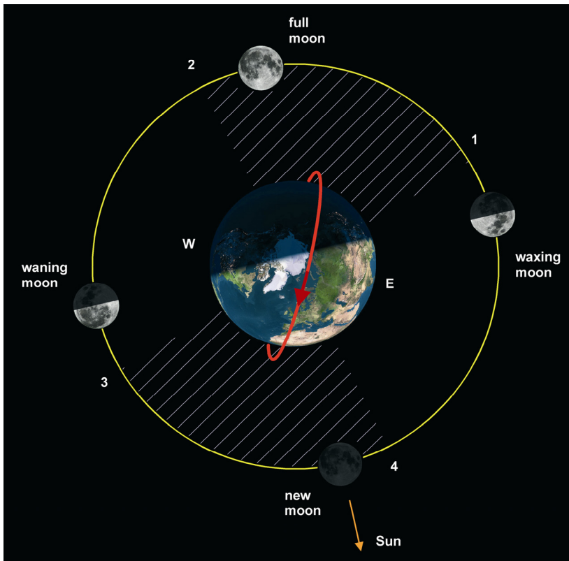
Fig. 4-5: SCIAMACHY's monthly lunar visibility occurs between 1 and 2 over the southern hemisphere (lunar phase > 0.5 ). The hatched area illustrates the limb TCFoV of 88^\circ . Visibility at smaller lunar phases over the northern hemisphere between 3 and 4 is not used because it coincides with solar occultations. (Courtesy: DLR-IMF)
