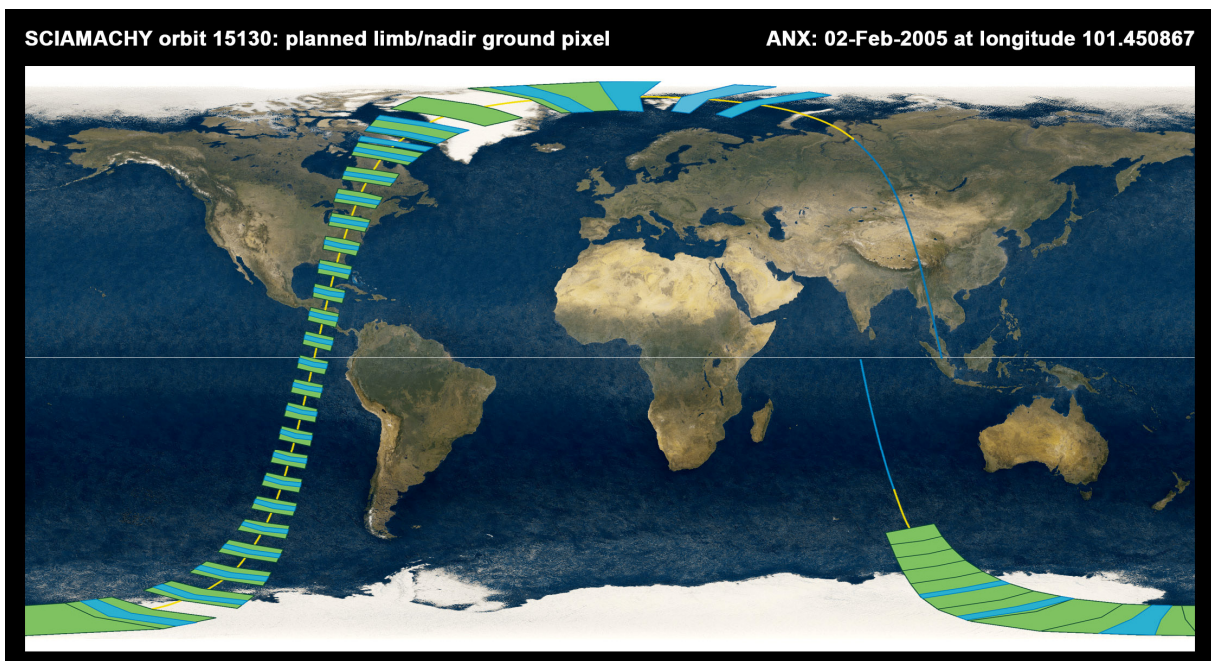
Fig. 4-2: An orbit with planned limb/nadir matching on the dayside of the orbit. The sequence of nadir and limb states in a timeline is arranged such that limb ground pixels (blue), defined by the line-of-sight tangent point, fall right into a nadir ground pixel (green) in the illuminated part of the orbit. (Courtesy: DLR-IMF/SRON)
