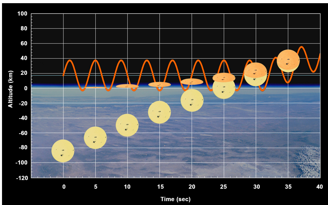
Fig. 4-6: The effect of refraction during sunrise. The position of the Sun is indicated by the yellow disk while the distorted refracted image appears above the horizon. About 30 sec after begin of sunrise the position of the true and refracted disk overlap and refraction becomes negligible. The sinusoidal curve illustrates the elevation scan of the ESM at the start of the Sun occultation states. (Courtesy: DLR-IMF; background photo: NASA Johnson Space Center and Image Science & Analysis Laboratory)
