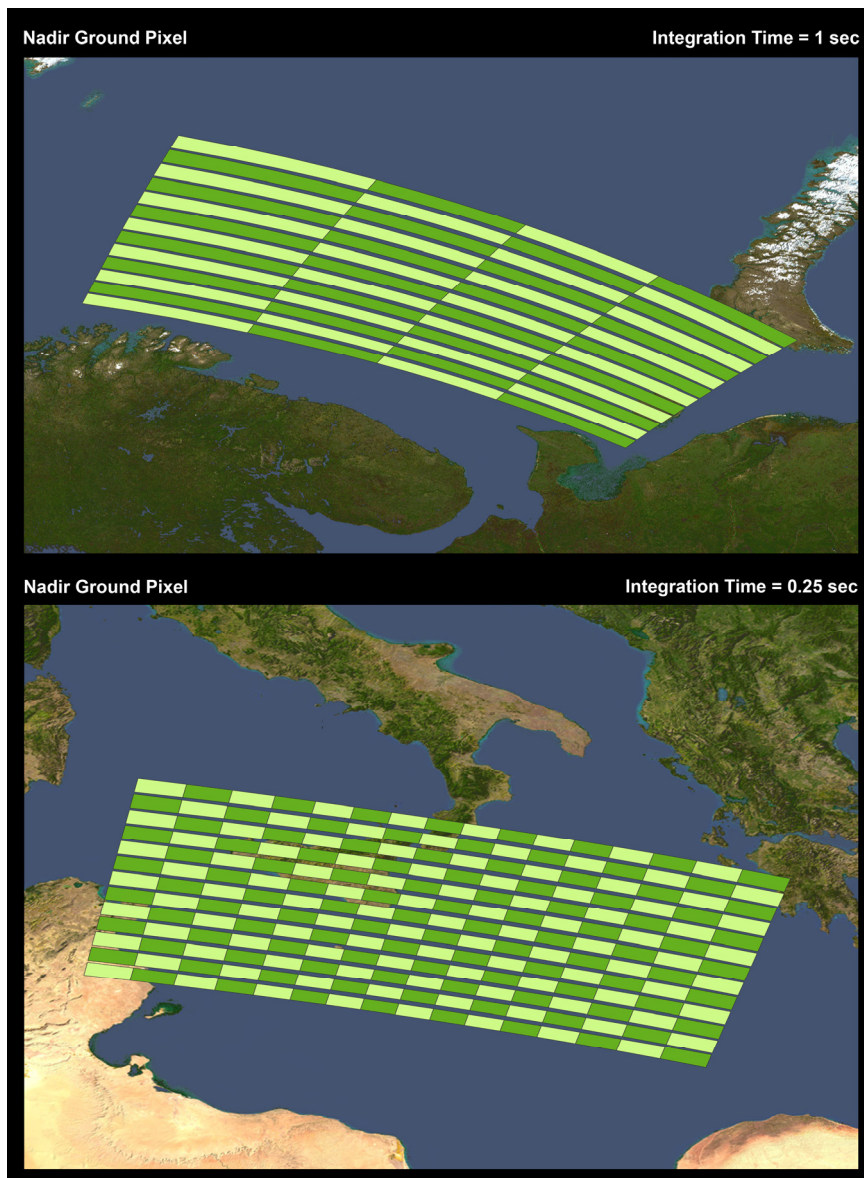
Fig. 4-9: The pattern of ground pixels in a nadir measurement for an integration time of 1 sec (top) and 250 msec (bottom). Only the forward scans are shown. This causes the along-track gaps between consecutive scans which vary in width due to a projection effect. Across-track extent is defined by the integration time while along-track the size reflects the dimension of the IFOV with only a small contribution of the integration time. (Courtesy: DLR-IMF; background maps: NASA)
