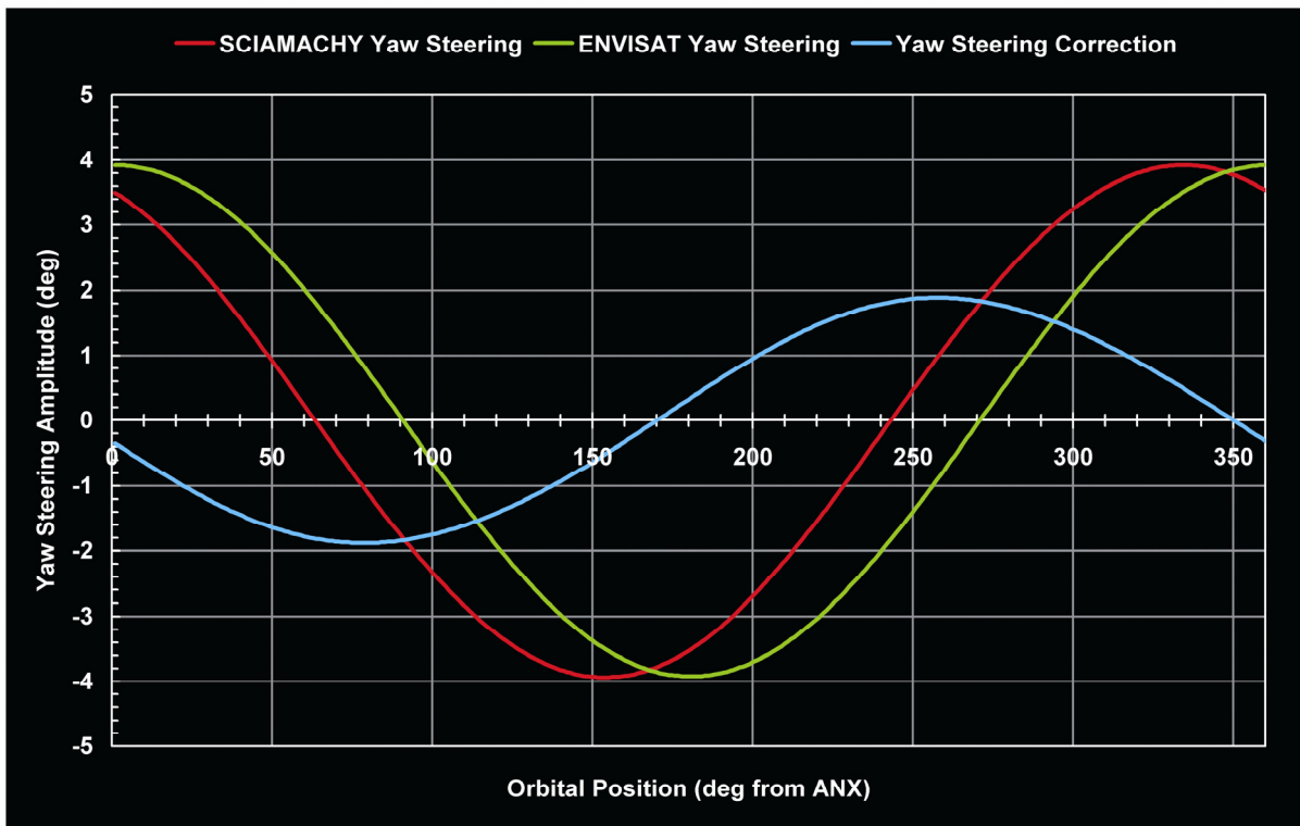
Fig. 4-3: ENVISAT's yaw steering, the yaw steering correction of limb states and the resulting SCIAMACHY yaw steering. Between ENVISAT and SCIAMACHY yaw steering, an orbital shift of 27° exists which reflects the observation geometry in elevation when looking to the horizon in flight direction. (Courtesy: DLR-IMF)
