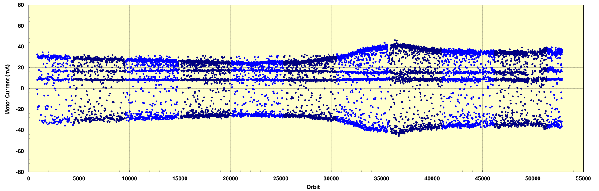
ESM Mean Motor Current - State 65
