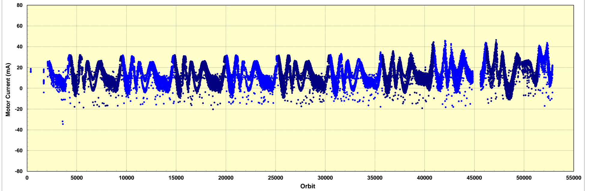
ASM Mean Motor Current - State 49
