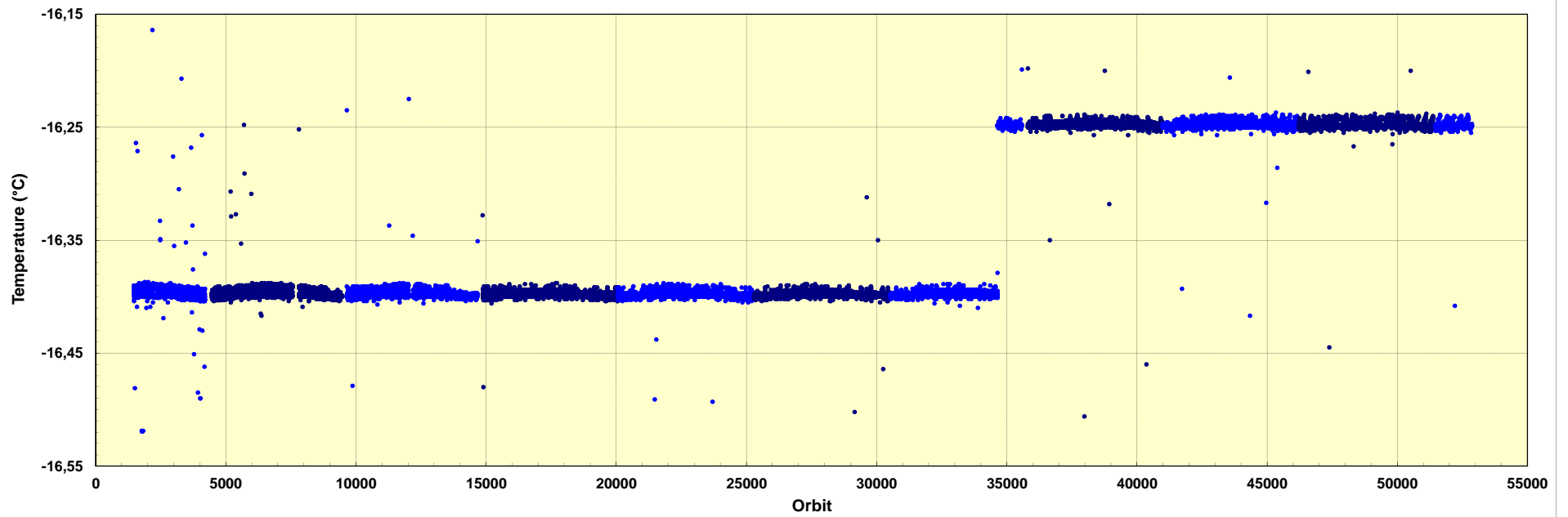
SCIAMACHY: ATC - Nadir Temperature
