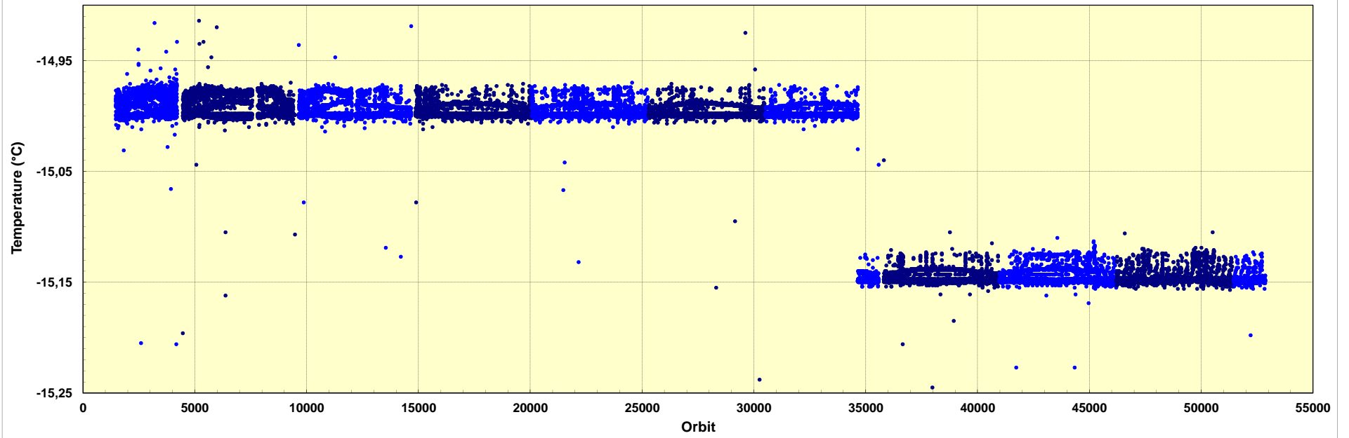
SCIAMACHY: ATC - Limb Temperature
