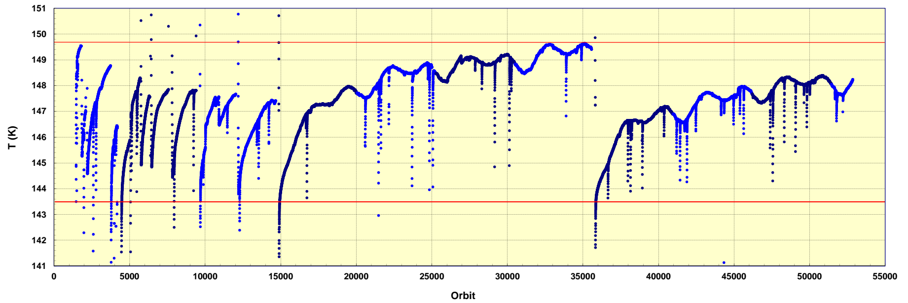
SCIAMACHY: Detector 8 Temperature
