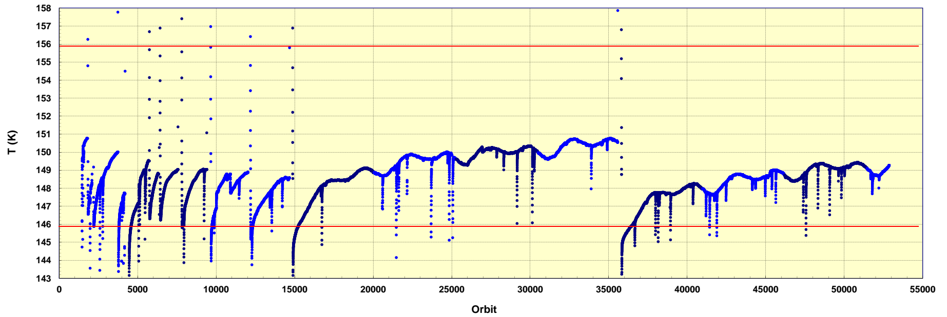
SCIAMACHY: Detector 7 Temperature
