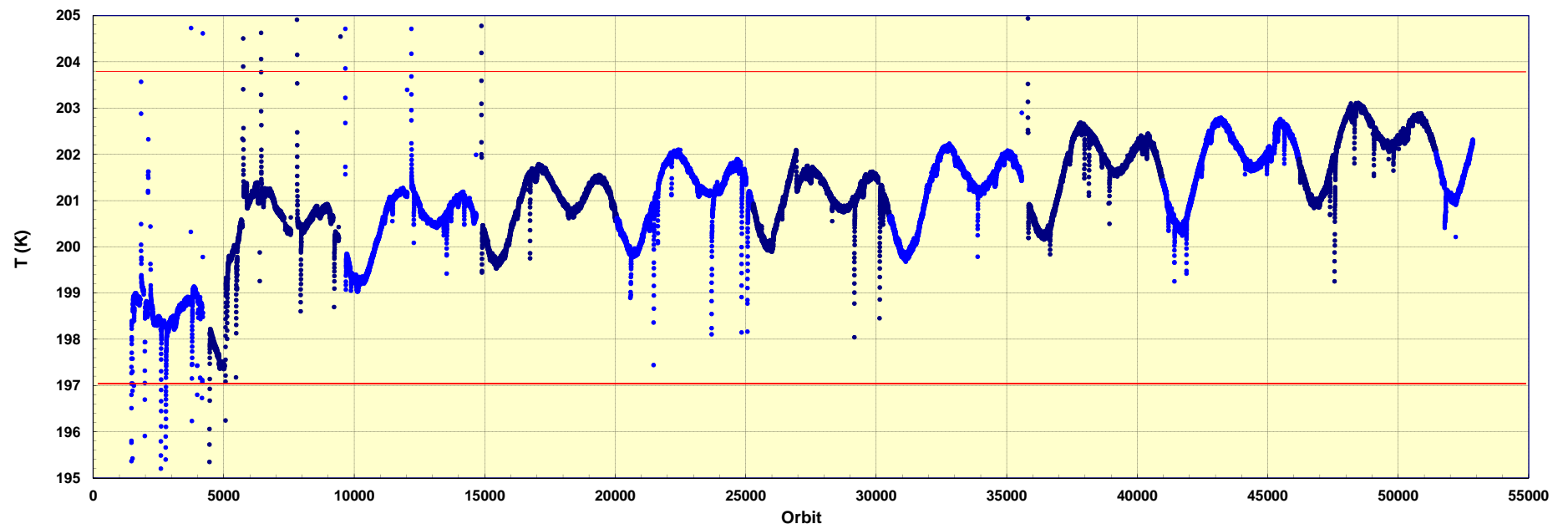
SCIAMACHY: Detector 6 Temperature
