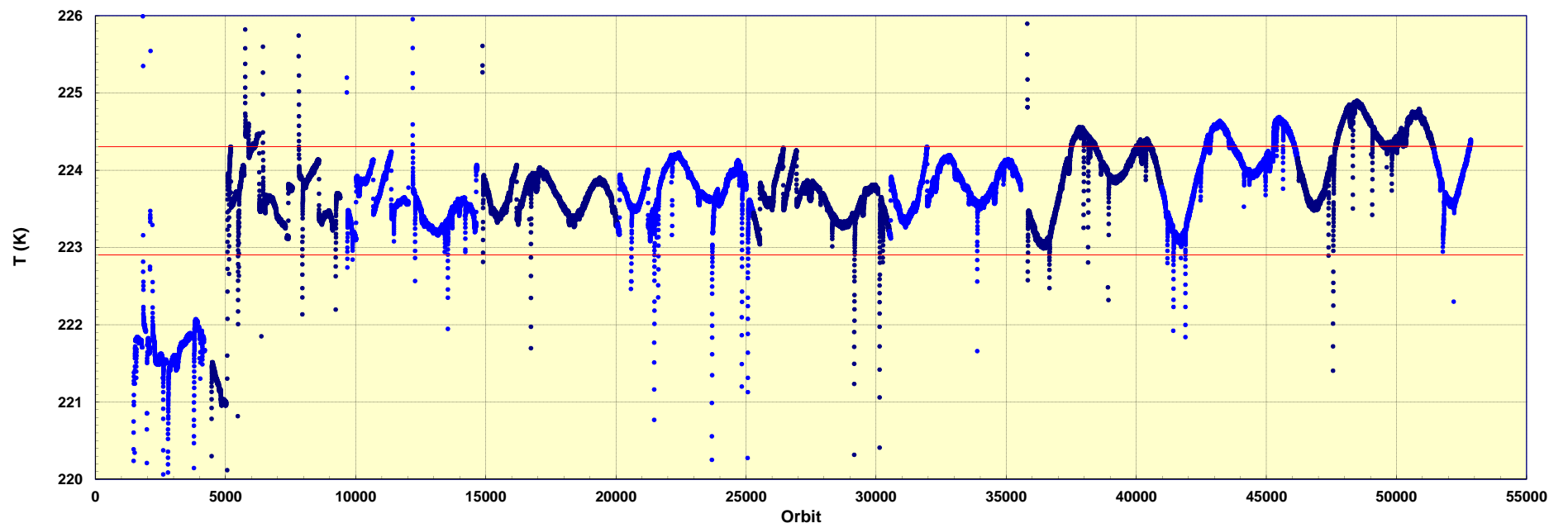
SCIAMACHY: Detector 4 Temperature
