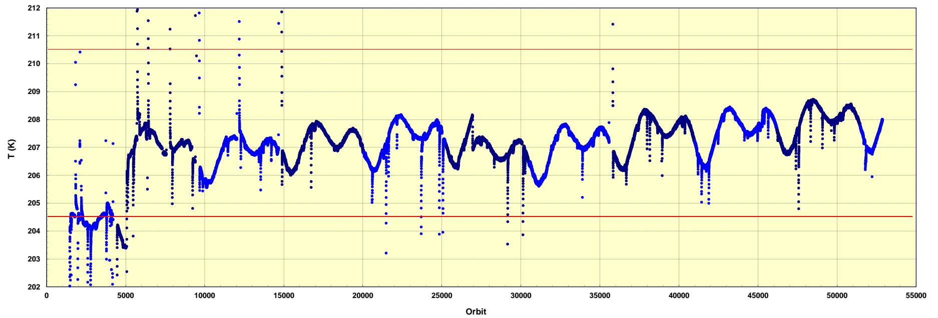
SCIAMACHY: Detector 1 Temperature
